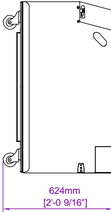
Side (With wheelboard attached)
